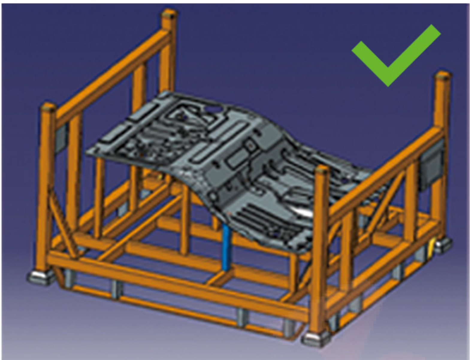
Stackable rack
