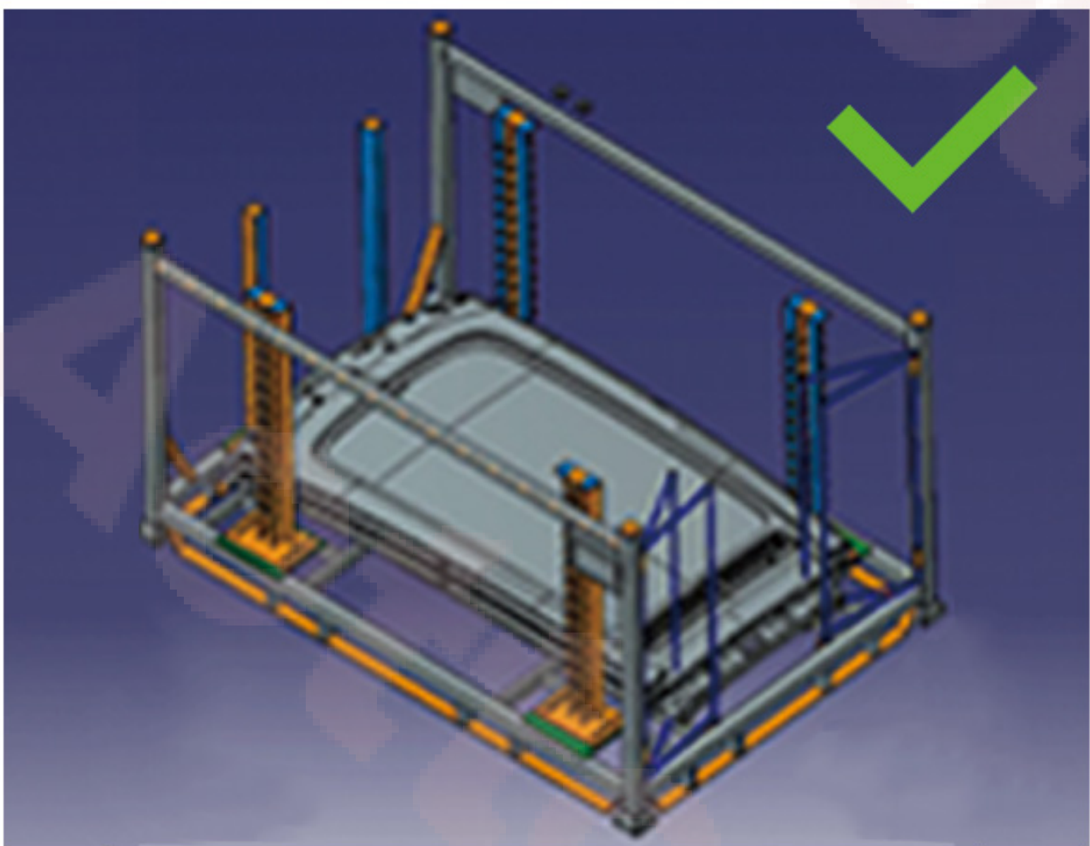
Flip-claw rack
